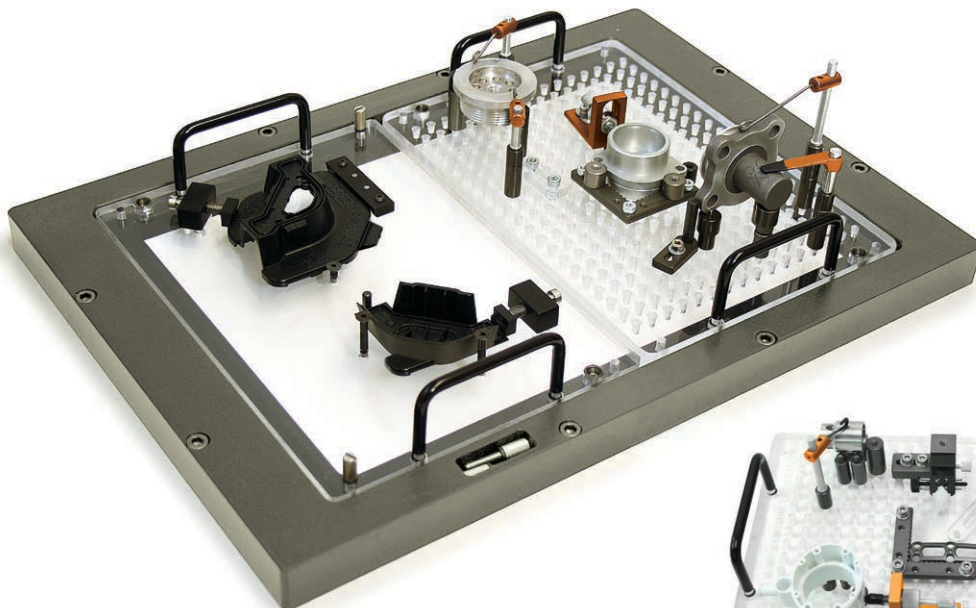
IVF(interchangeable vision fixture)
