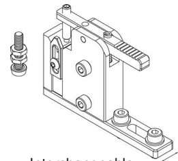
Interchangeable clamp inserts
